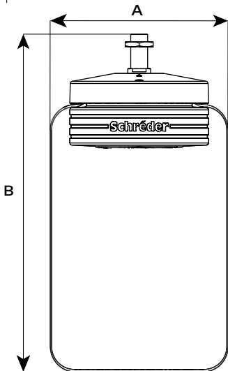
SUSPENDED VERSION
