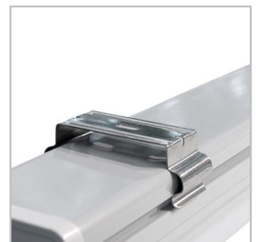
A versatile installation system enables surface (fixed or pendant) or wall mounting.
